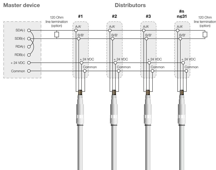
Figure 19: Wiring diagram for the RS485 interface
